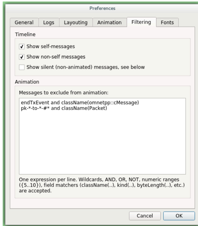
Figure 7.32. Filtering
