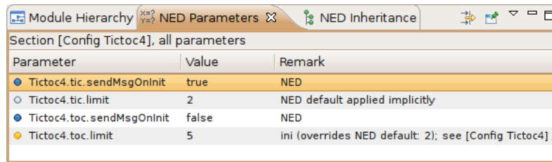
Figure 3.10. Parameters View
