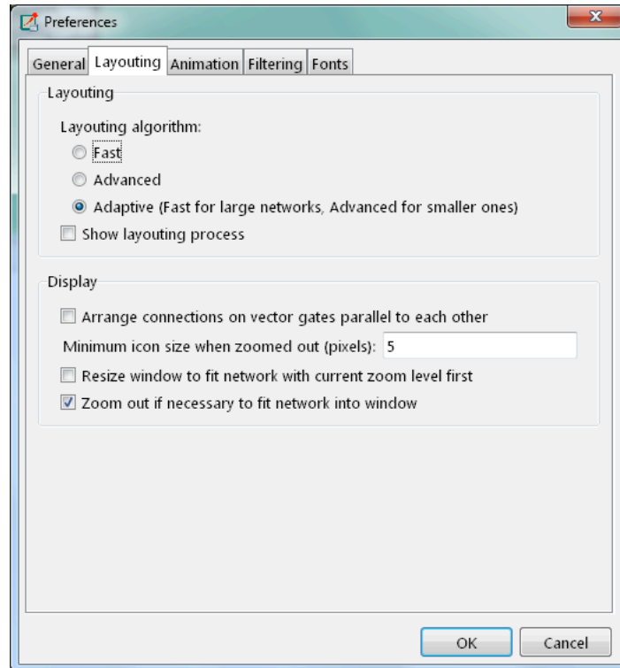
Figure 8.26. Layouting settings
