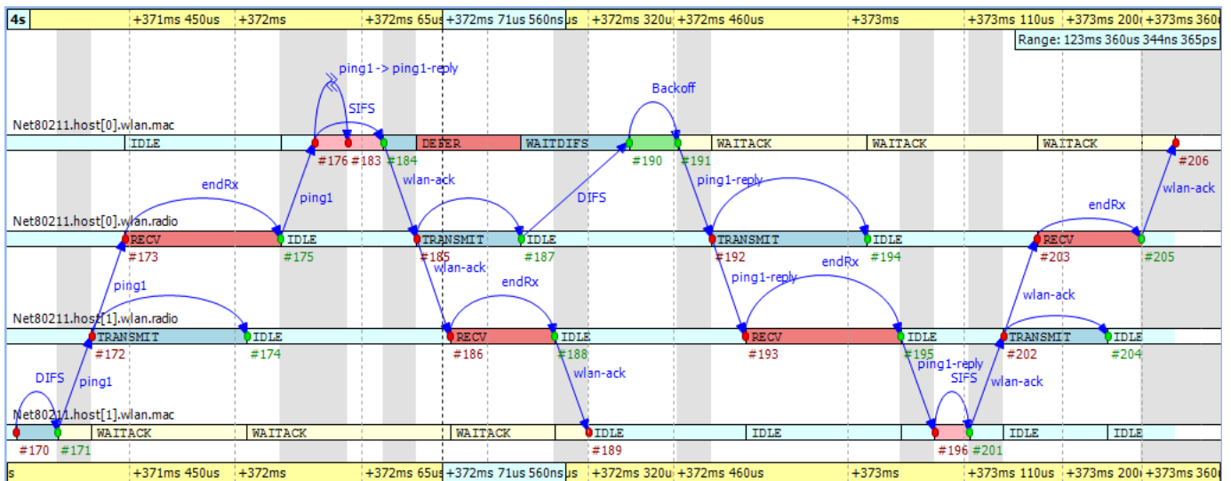
Figure 9.26. The second ping procedure
